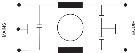
CIRCUIT DIAGRAM
