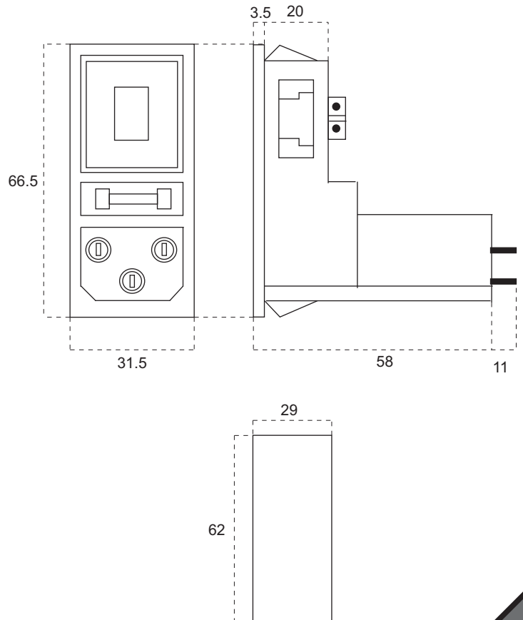
PANEL CUTOUT
