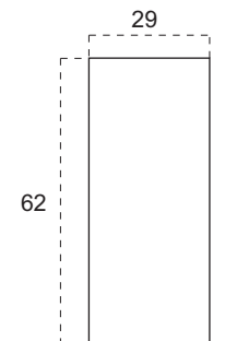
PANEL CUTOUT
