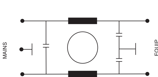
CIRCUIT DIAGRAM
